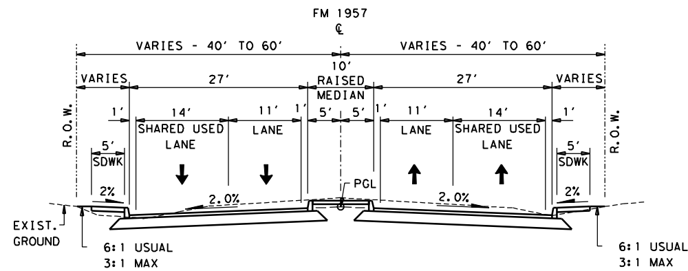
PROPOSED RAISED MEDIAN TYPICAL SECTION
