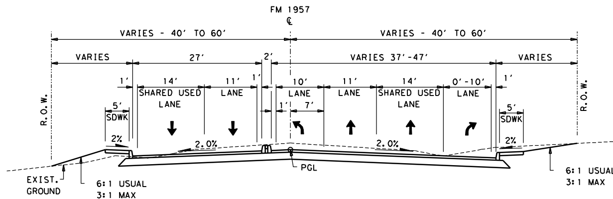
PROPOSED LT & RT TURN TYPICAL SECTION
